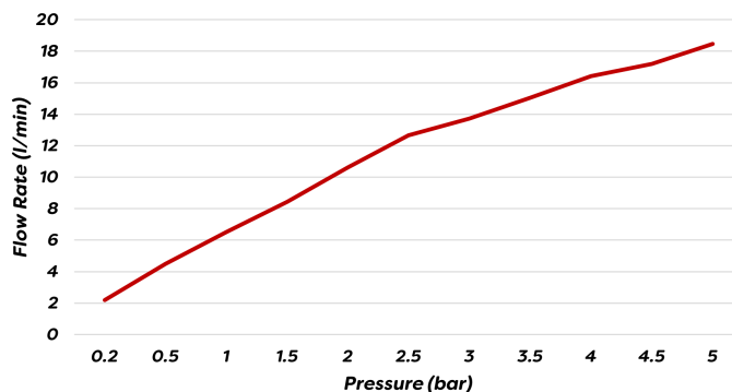
IX400014CP Flow Rate
