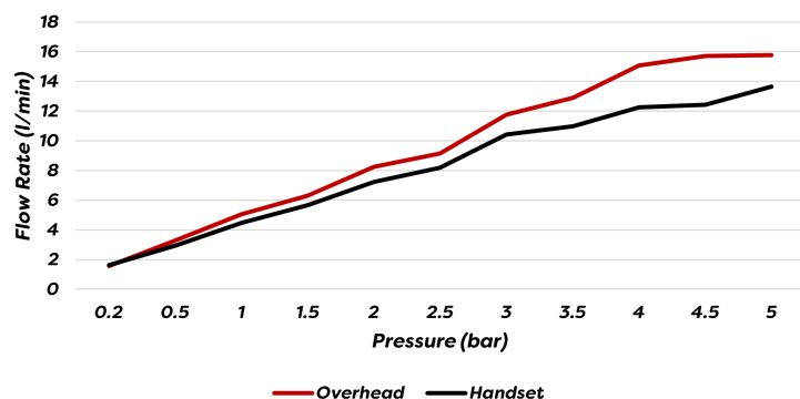
IX200025BK Flow Rate
