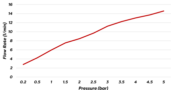
IX100010CP Flow Rate
