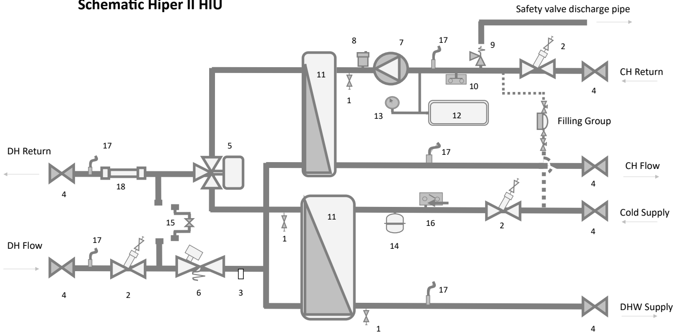
Schematic Hiper II HIU
