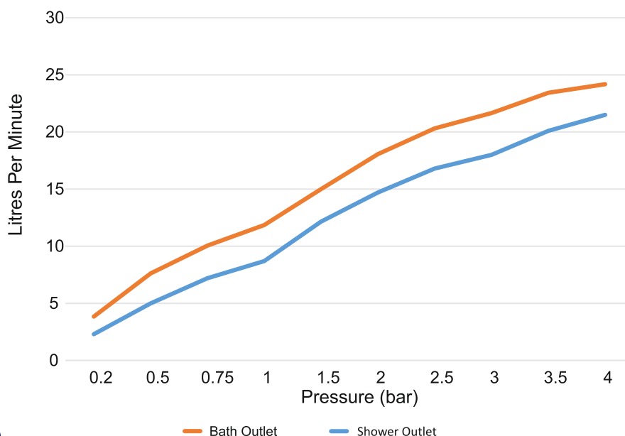
Flow Rate Graph
