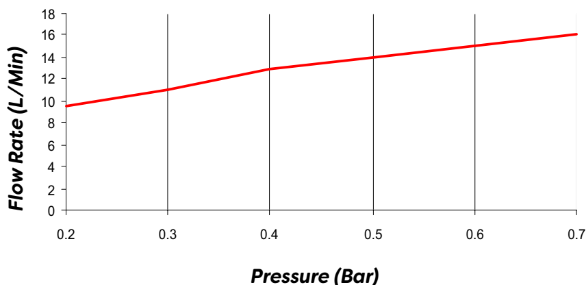
VR992CP Flow Rates
